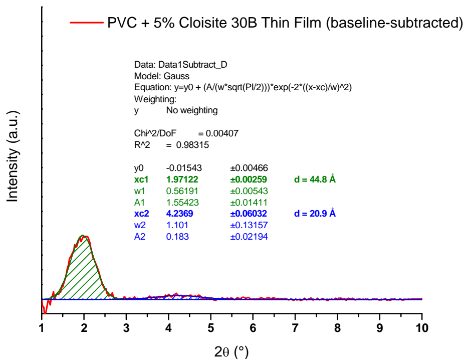
Figure 9. Integrated intensity (arbitrary units) vs. 2\theta (°), baseline-subtracted and peak-fit using a Gaussian model, for Bse nanocomposite sheet
