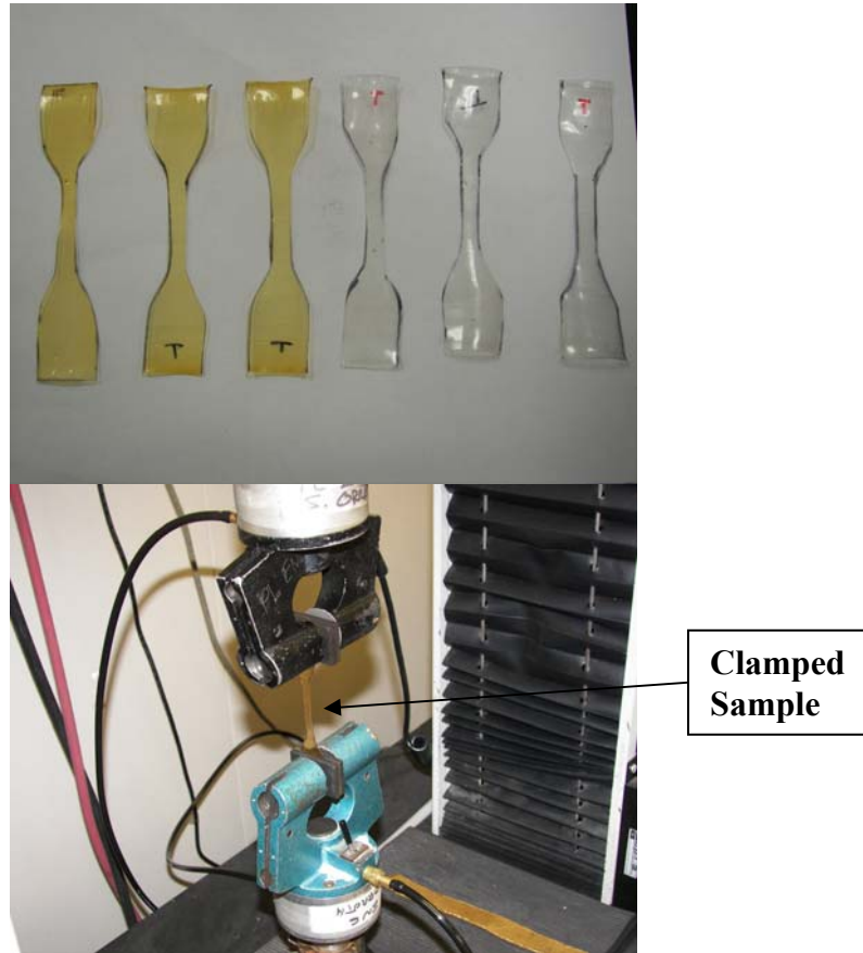
Figure 13. Sample Ase cut tensile and Sample Jse (virgin PVC) cut tensile (at right).
