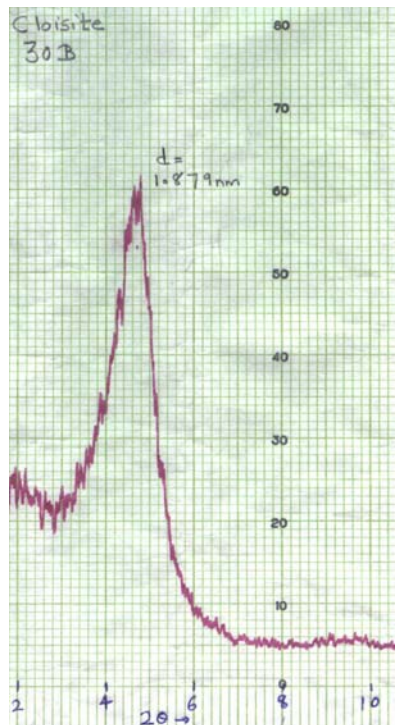
Figure 4. XRD Pattern of Clay1 (Pure Cloisite 30B)
