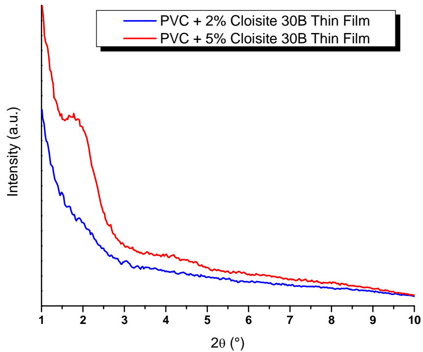
Figure 7. Integrated intensity (arbitrary units) vs. 2\theta ( ^{\circ} ) for PVC NC thin films samples Ase (blue) and Bse (red).
