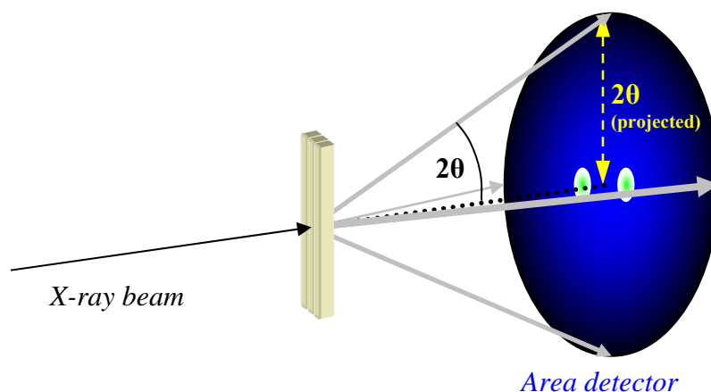
Figure 3. Schematic of Transmission Geometry XRD with Area Detector
