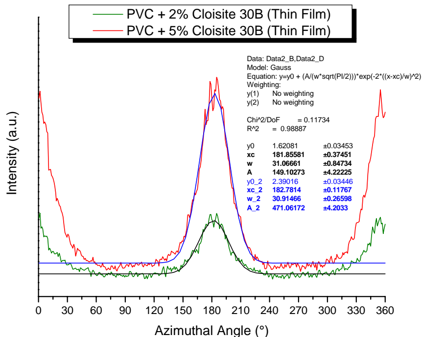
Figure 10. Azimuthal scans for PVC nanocomposite sheets Ase and Bse
