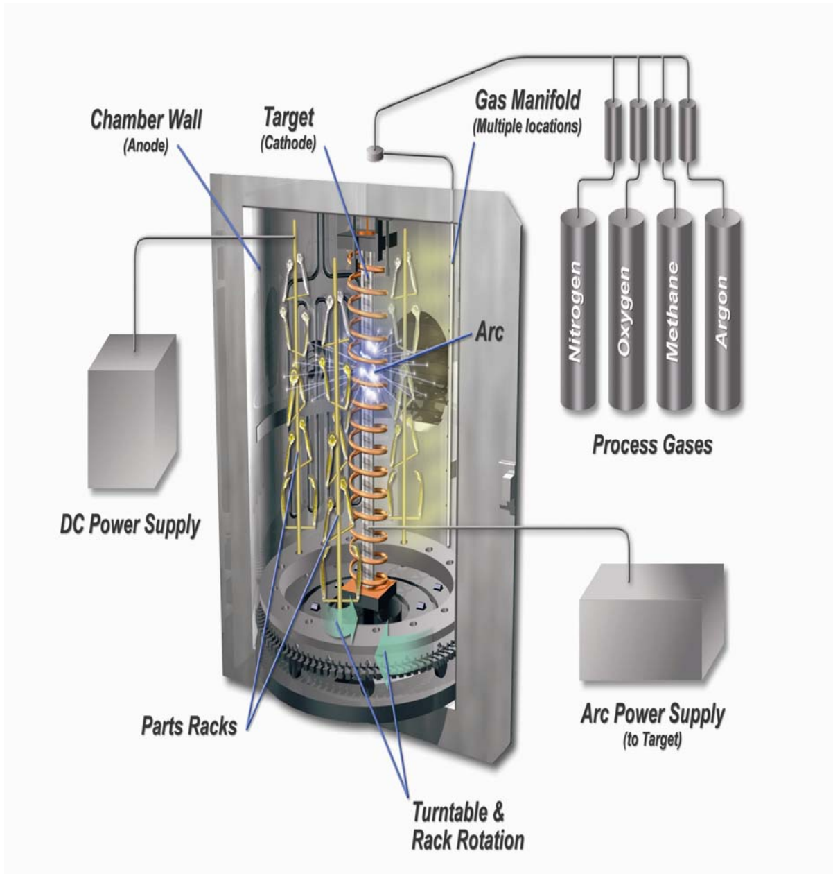
Figure 6.4.1 D: Low Temperature Arc Vapor Deposition (LTAVD®) Process (Diagram reproduced courtesy of Vapor Technologies, Longmont, CO)
