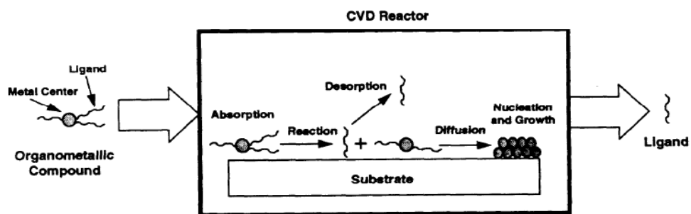
Figure 6.4.2 C: Chemical Vapor Deposition (NDCEE 1995)
