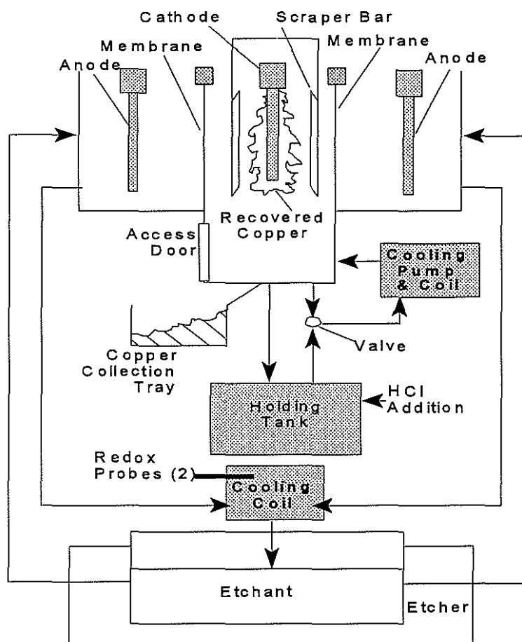
Figure 1: Cupric Chloride Electrolytic Regeneration Cell
